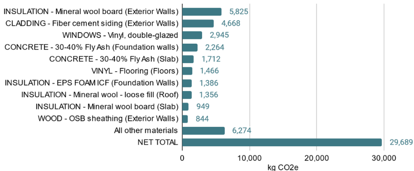
Figure 11 Top 10 highest-ranking carbon-intensive building materials in Tier 4, Two Storey house in Toronto as per the MCM selection
